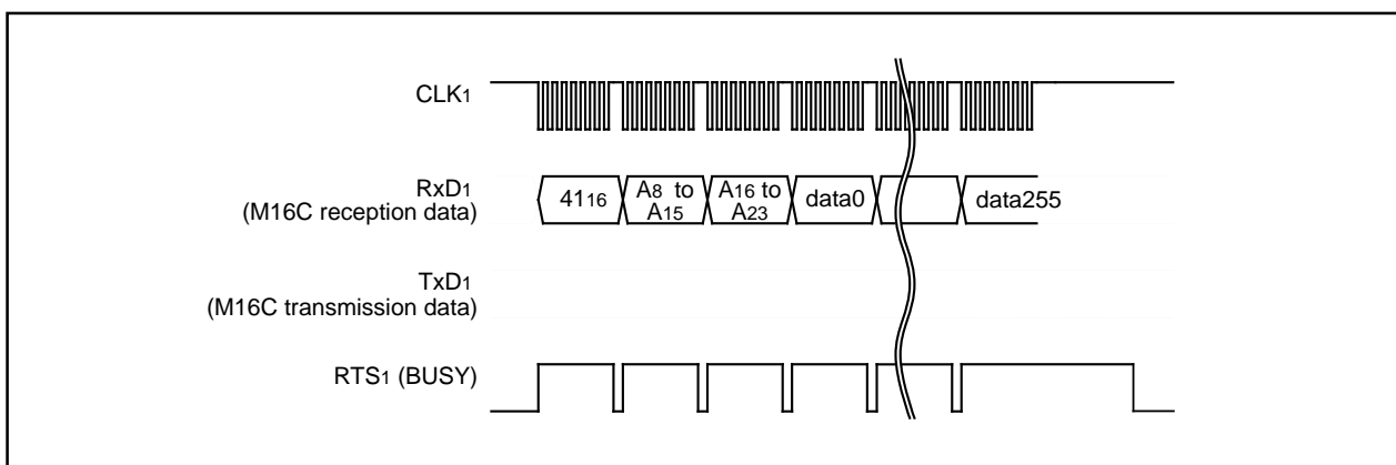
Figure 1.28.2. Timing for the page program
